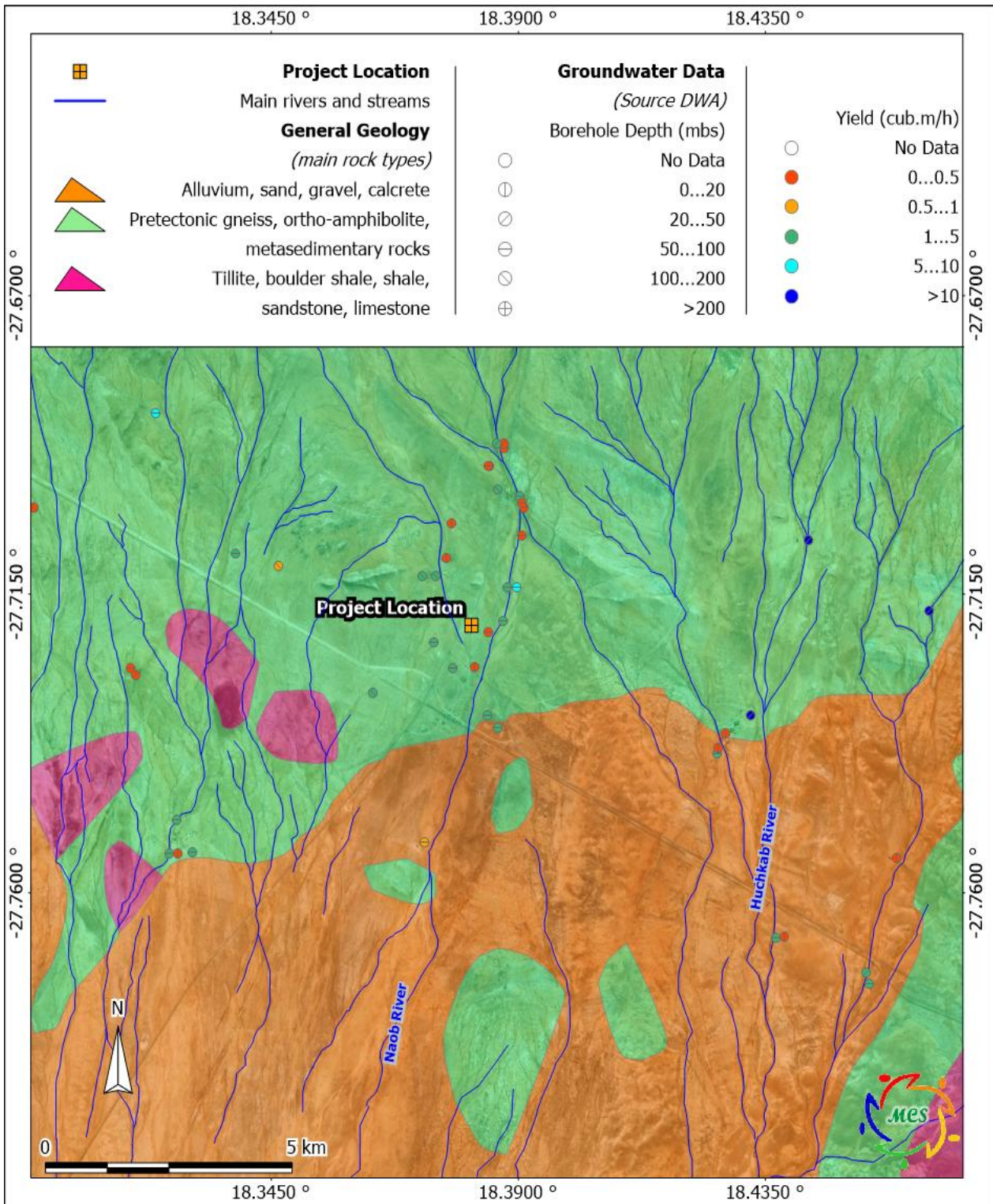
Figure 3. Hydrogeology of the area
