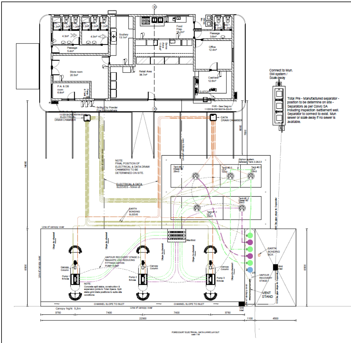
Figure 2. Proposed new layout plan of the facility
