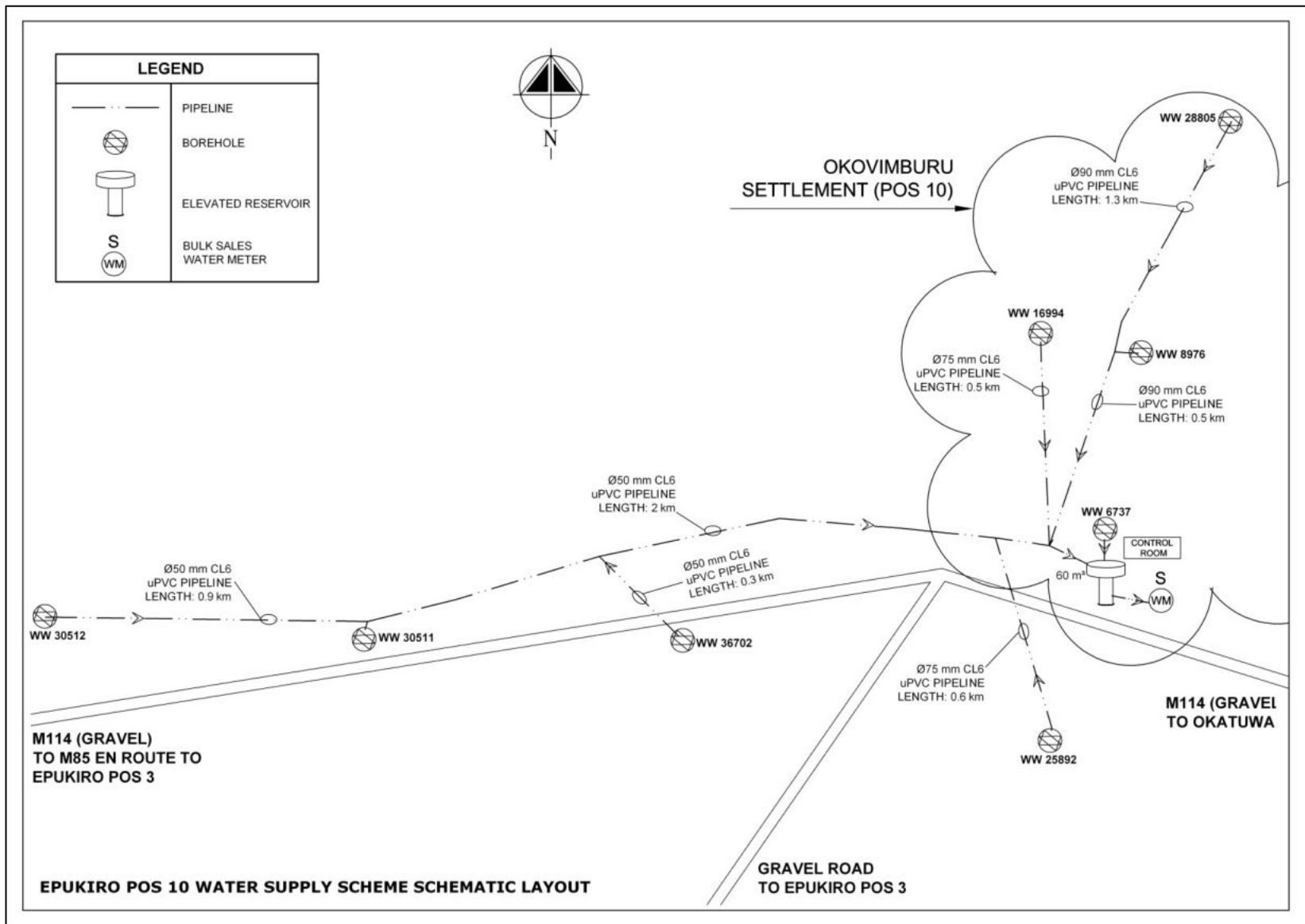
Figure 3: Epuikiro Pos 10 Scheme Layout
