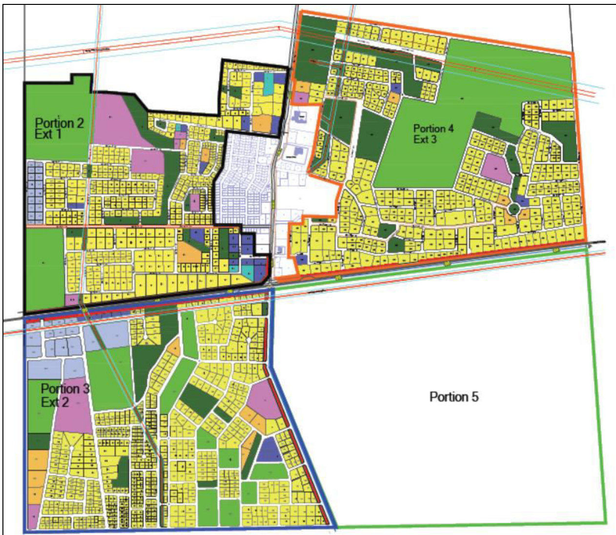
Figure 1: Ndiyona Extension 1, 2 & 3 Layout
