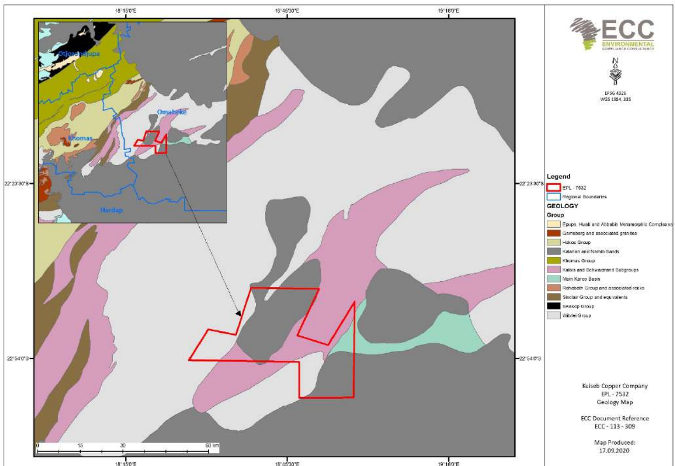
FIGURE 5 - REGIONAL GEOLOGICAL SETTING OF EPL 7532
