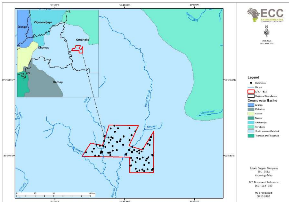
FIGURE 8 - REGIONAL HYDROLOGY MAP OF EPL 7532
