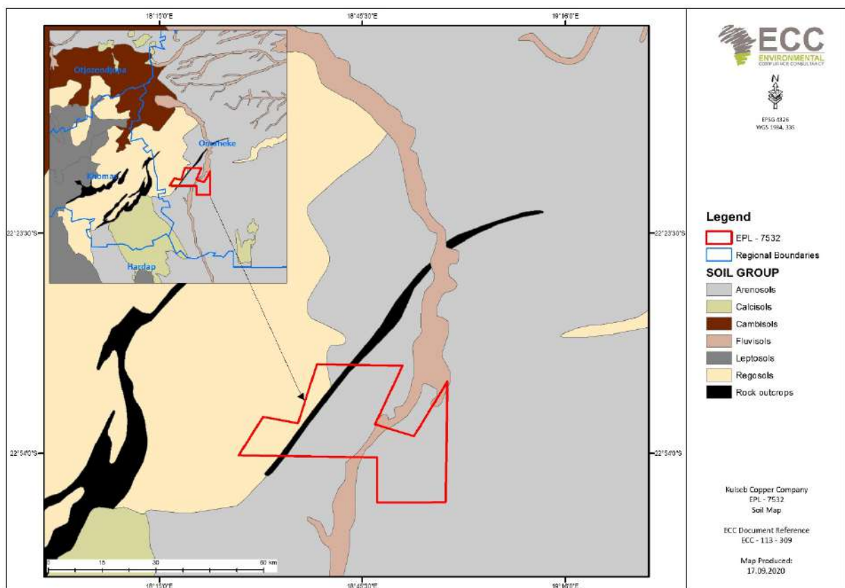
FIGURE 7 - REGIONAL SOIL MAP OF EPL 7532
