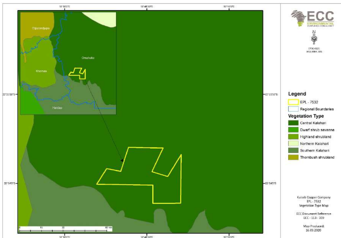
FIGURE 9 - REGIONAL VEGETATION MAP OF EPL 7532
