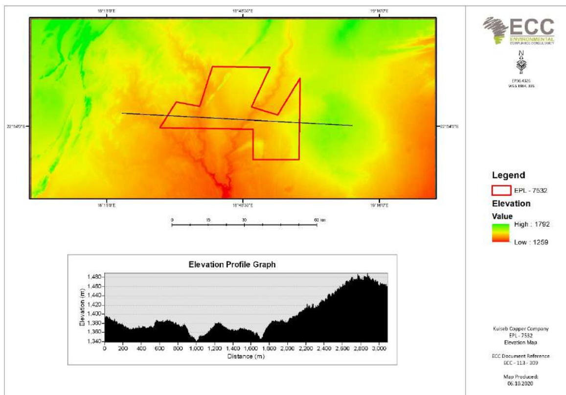
FIGURE 6 - ELEVATION PROFILE FOR EPL 7532
