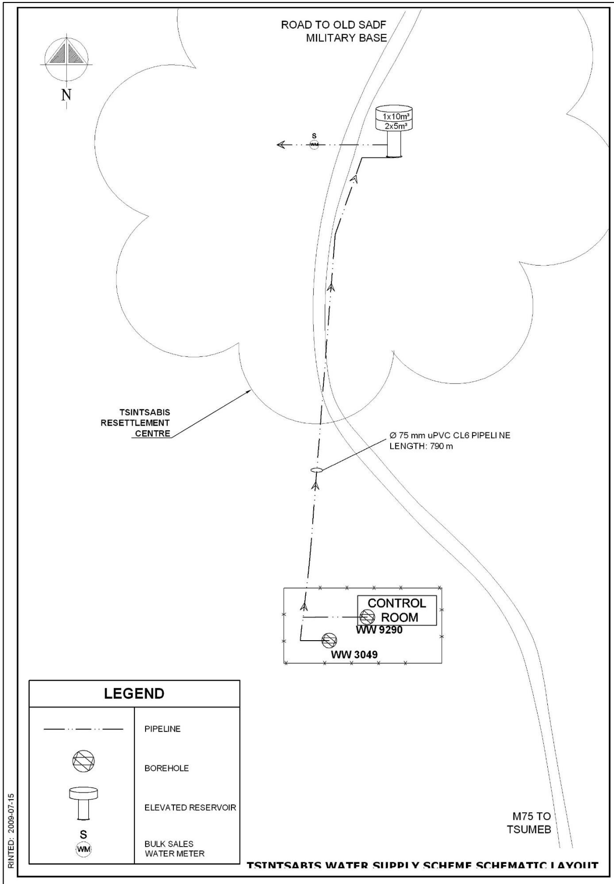
Figure 2: Tsintsabis Scheme Layout
