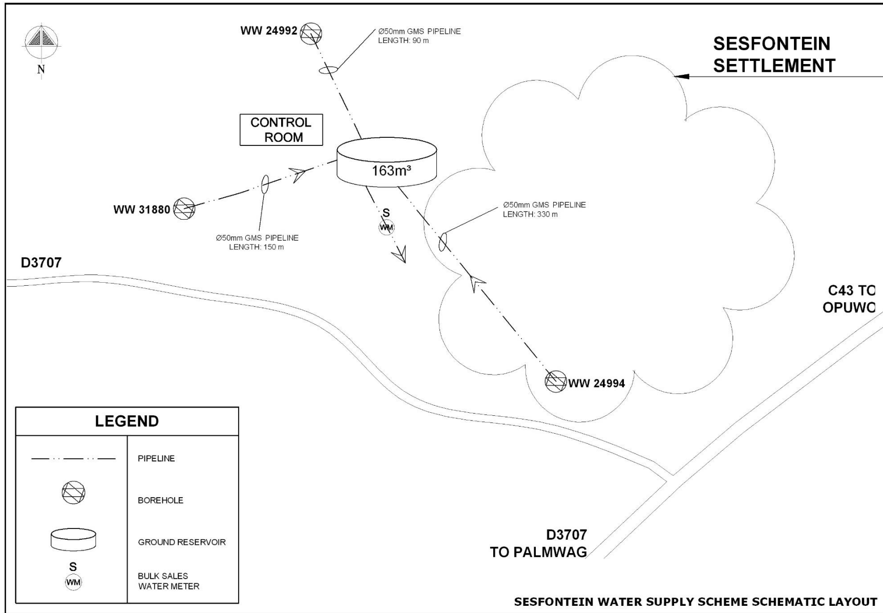
Figure 2: Sesfontein Scheme Layout
