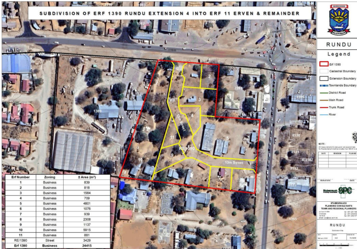
Figure 3: Aerial Map of proposed Subdivision of Erf 1390, Rundu Extension 4.
