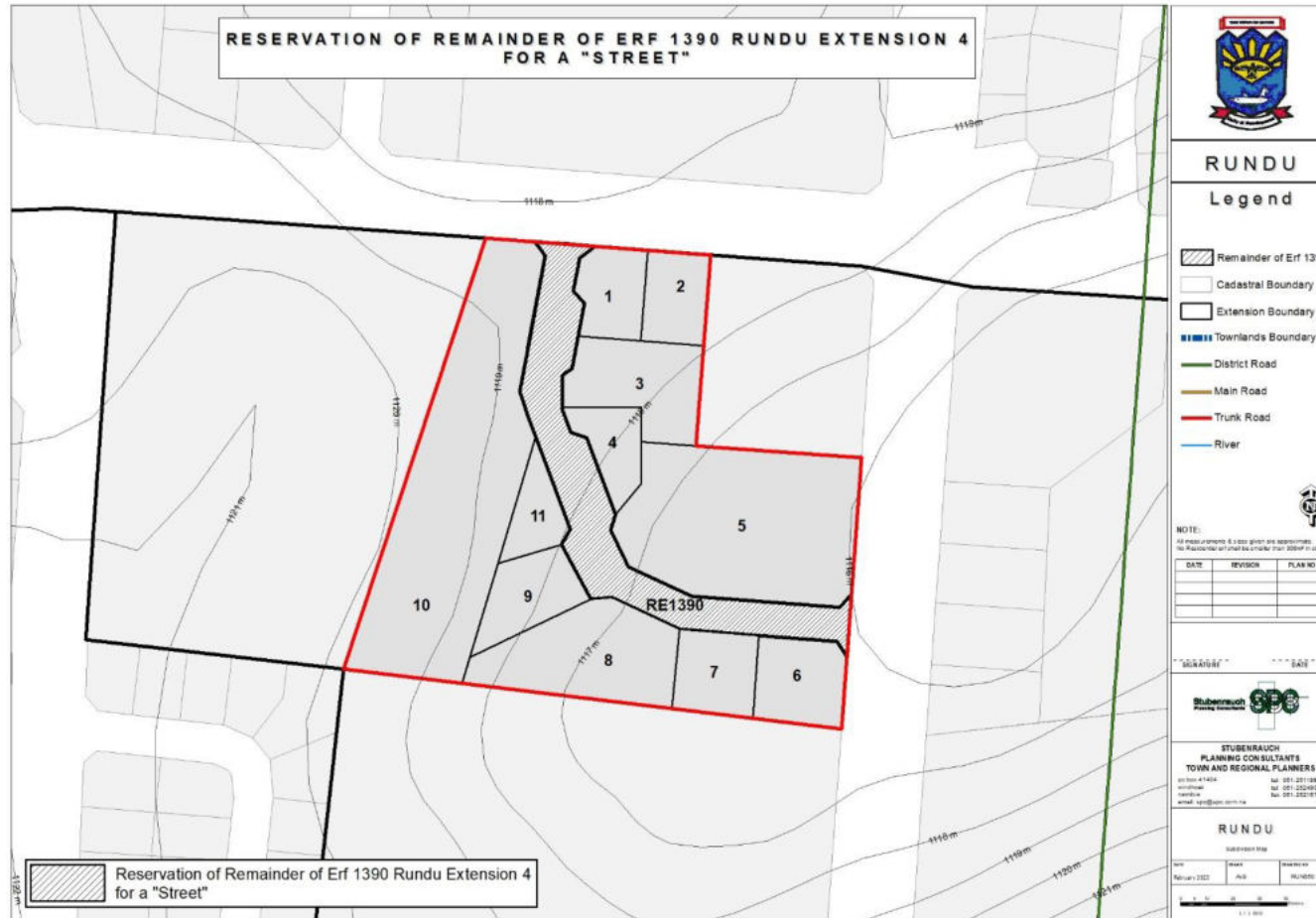
Figure 4: Reservation of Remainder of Erf 1390 Extension 4 for a Street.
