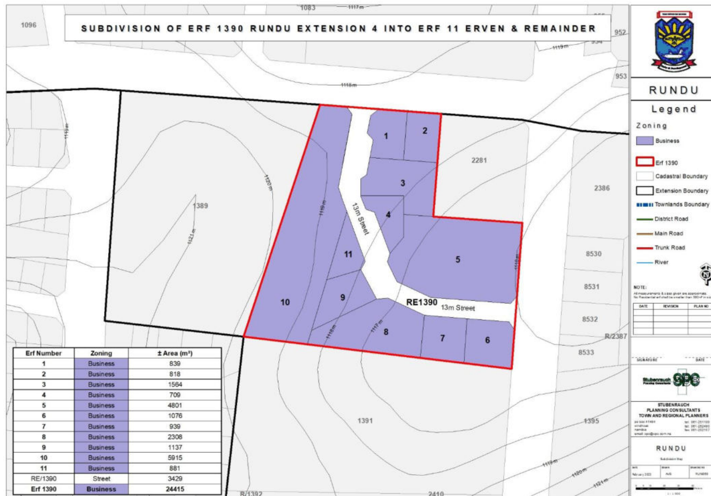
Figure 2: Layout map of the Proposed Subdivision of Erf 1390 Rundu Extension 4 into 11 Erven and Remainder.
