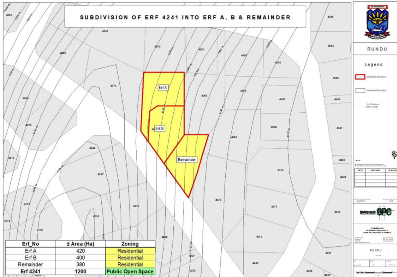
Figure 4: Layout map for the proposed Subdivision of Erf 4241, Kaisosi Extension 12.
