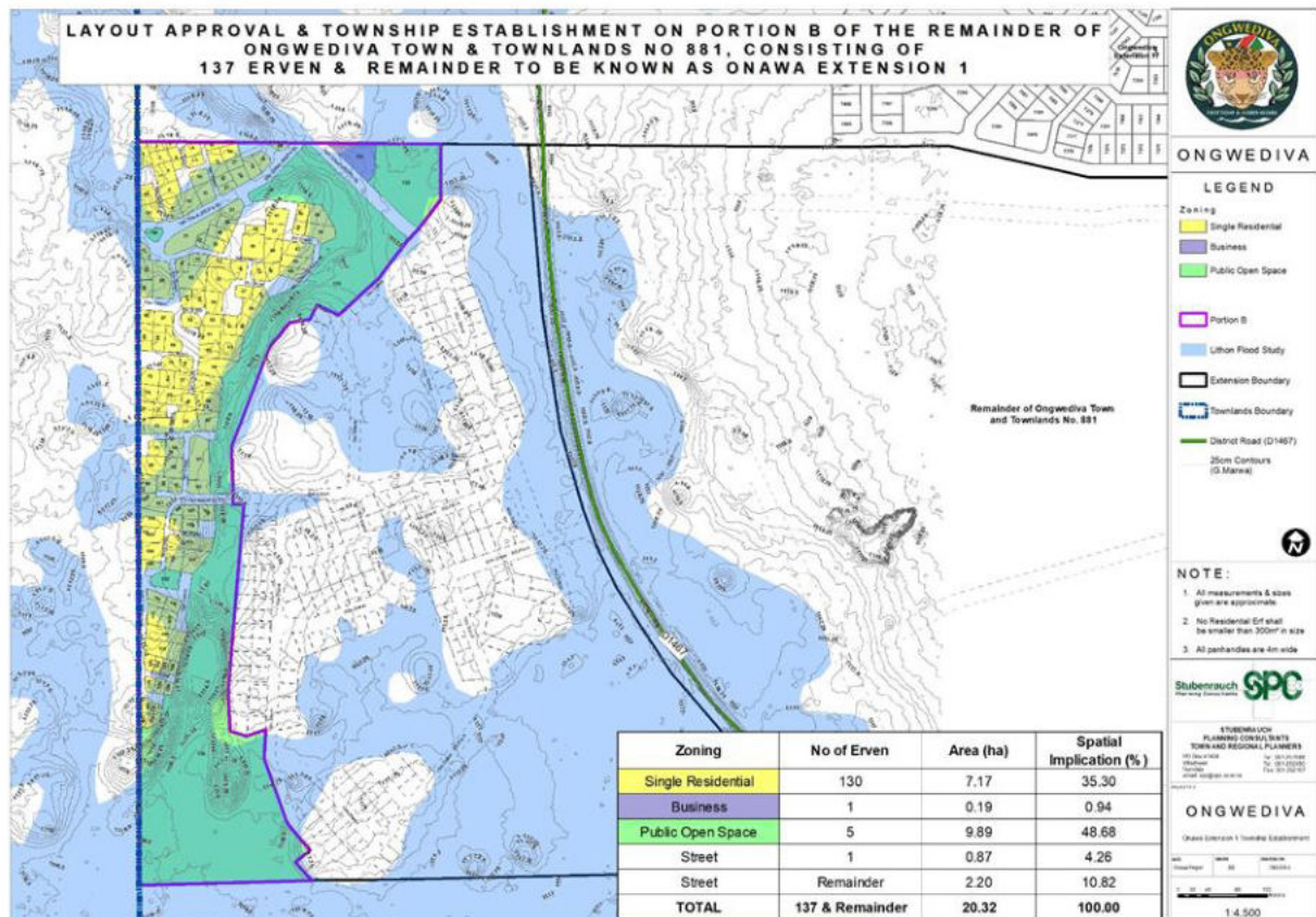
Figure 3: Layout of Proposed Onawa Extension 1
