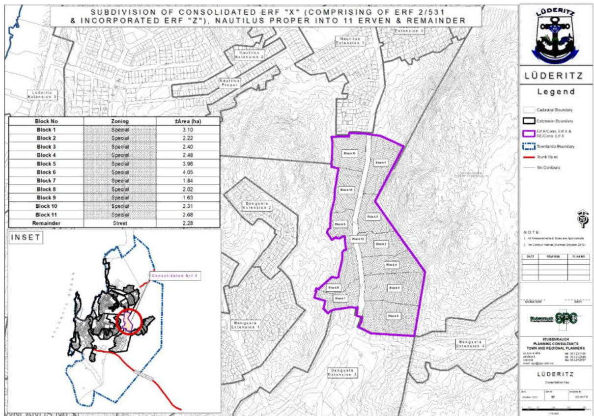
Figure 7: Subdivision of Consolidated Erf X into 11 blocks and the Remainder
