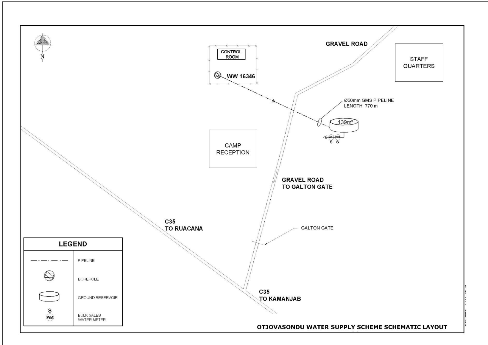
Figure 2: Otjovasandu Scheme Layout
