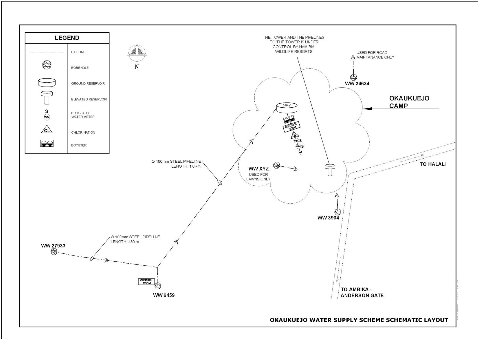
Figure 2: Okaukuejo Scheme Layout
