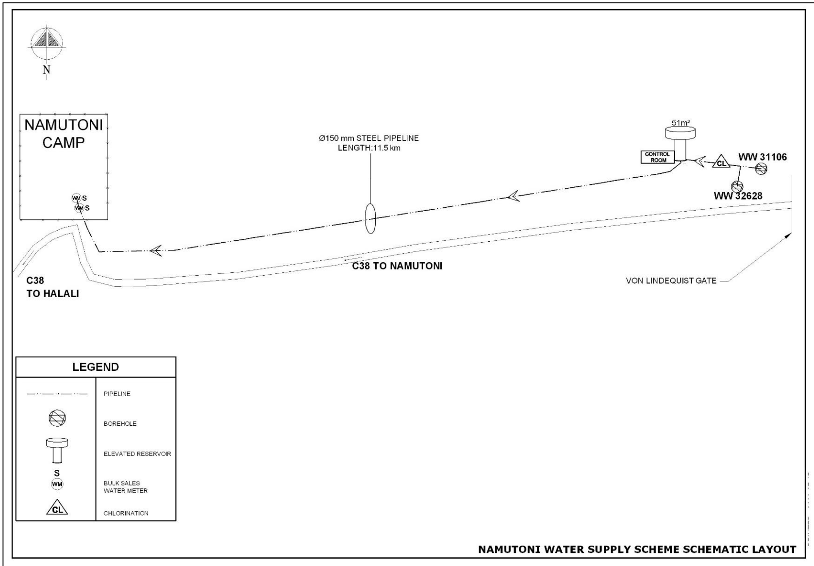
Figure 2: Namutoni Scheme Layout
