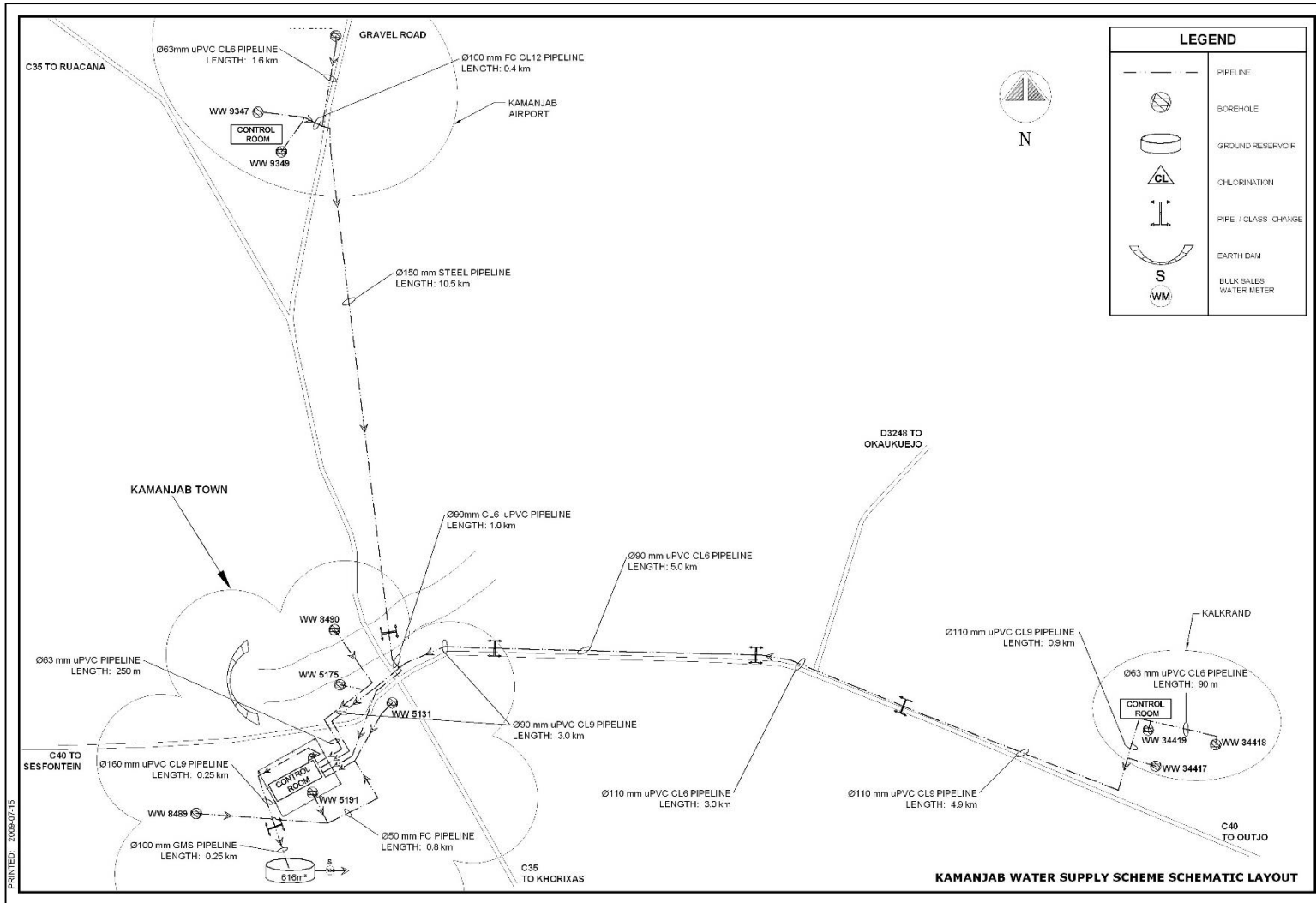
Figure 2: Kamanjab Scheme Layout
