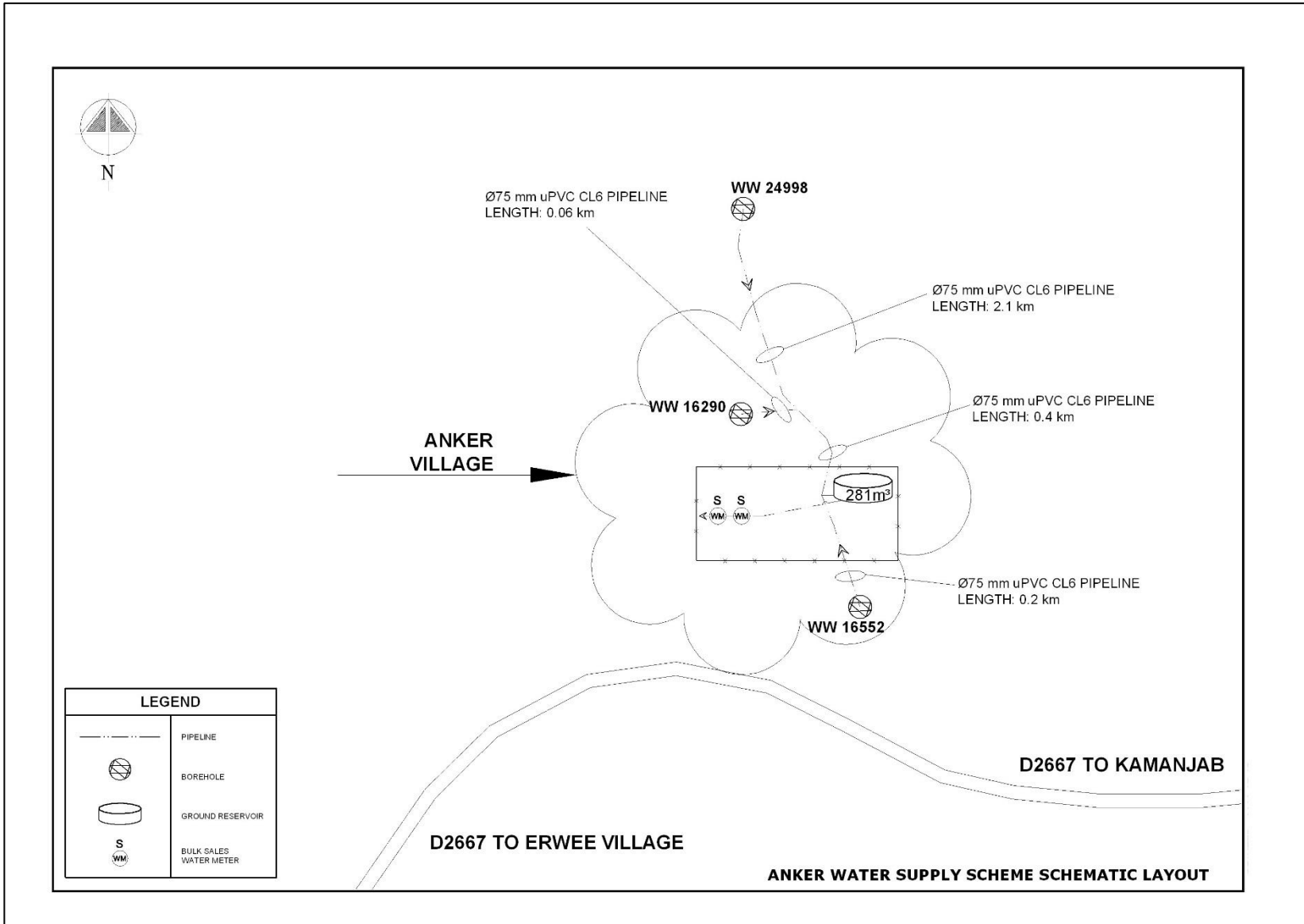
Figure 2: Anker Scheme Layout
