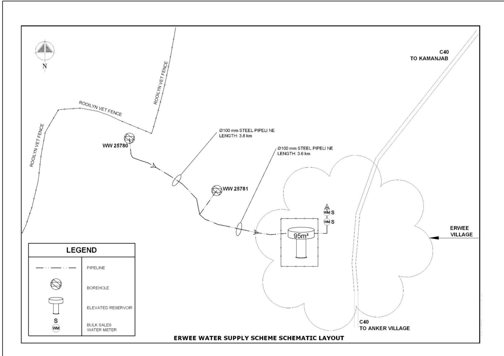
Figure 2: Erwee Scheme Layout
