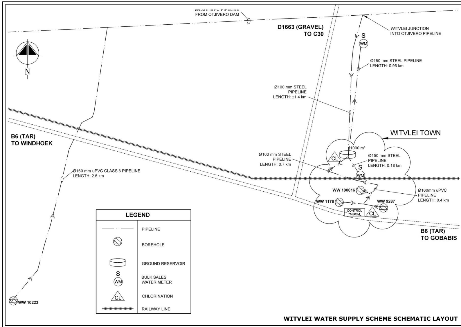
Figure 2: Witvlei Scheme Layout
