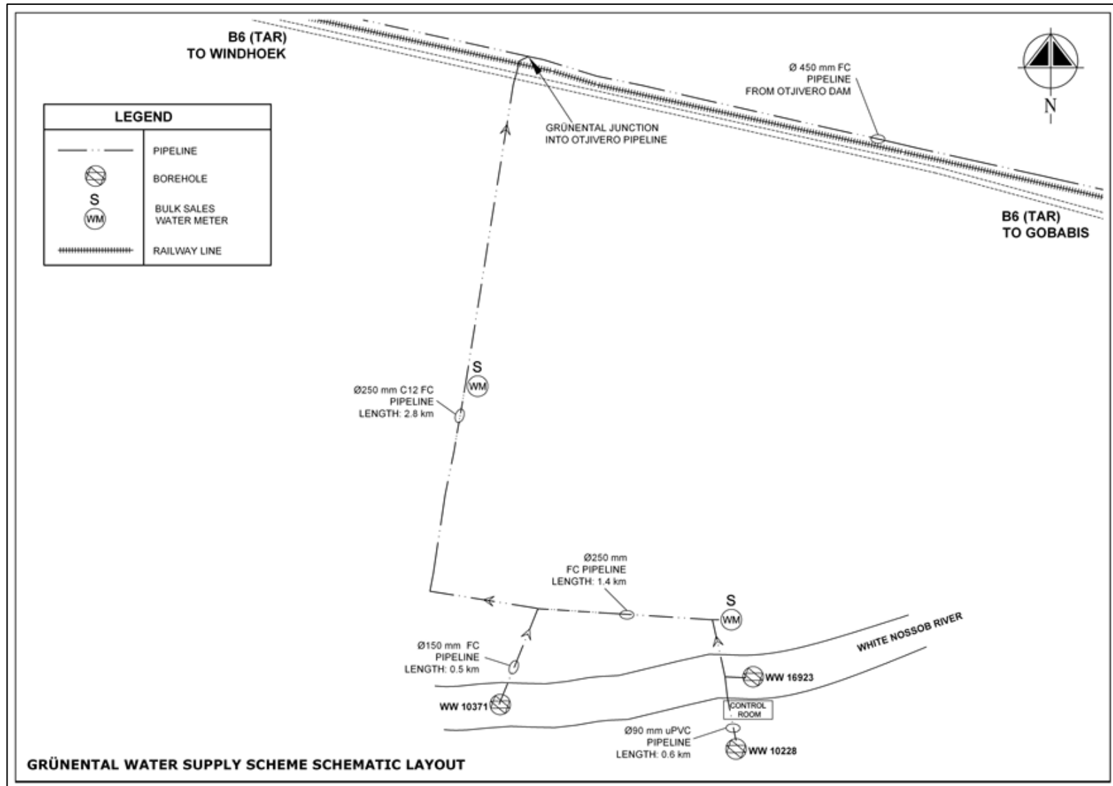
Figure 3: Grünental Scheme Layout
