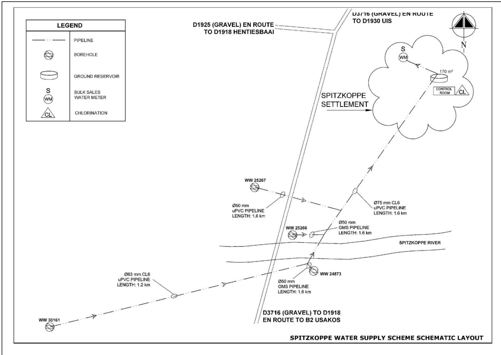
Figure 2: Spitzkoppe Scheme Layout
