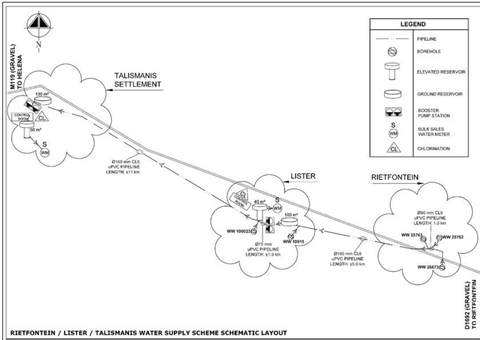
Figure 2: Rietfontein-Lister-Talismanis Scheme Layout
