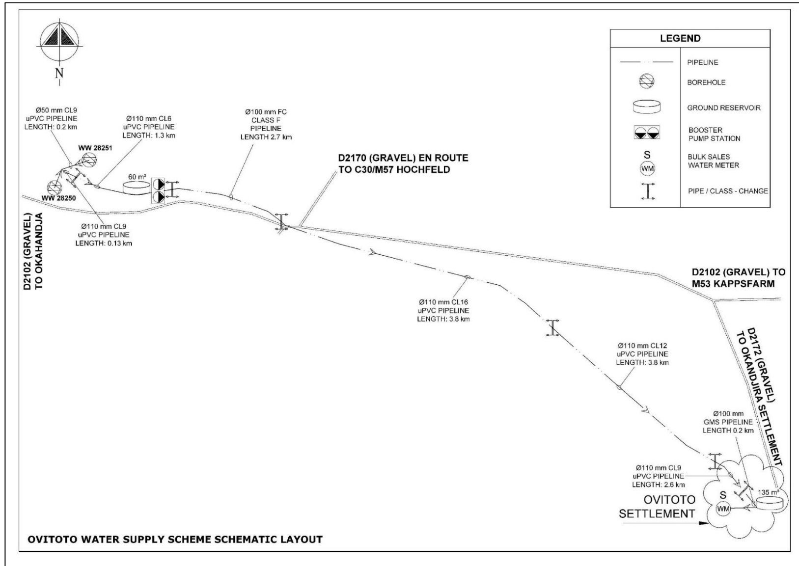
Figure 2: Ovitoto Scheme Layout
