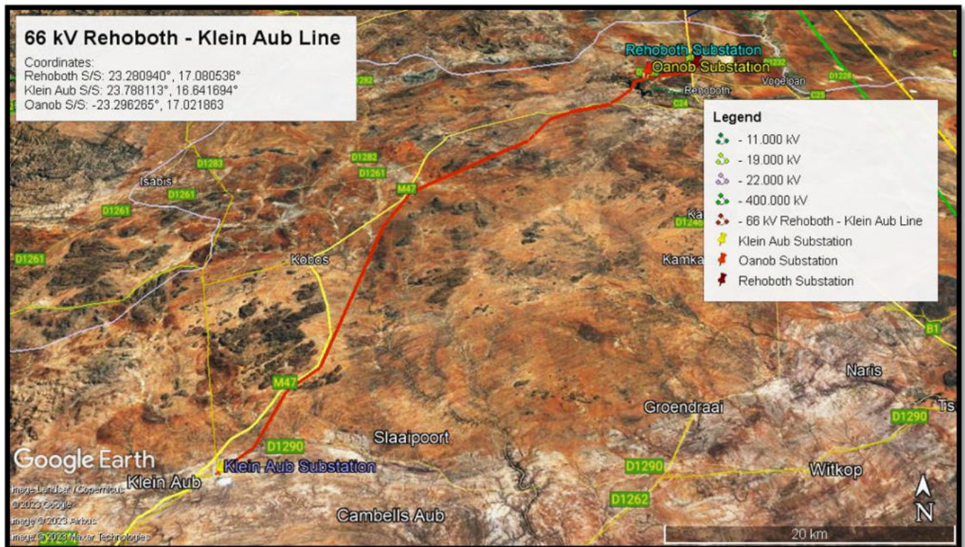
Figure 1: Locality map showing the 66 kV Rehoboth- Klein Aub transmission line
