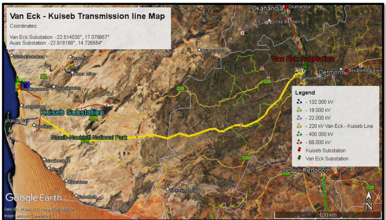
Figure 1: Locality map showing the 220kV Van Eck – Kuiseb transmission line
