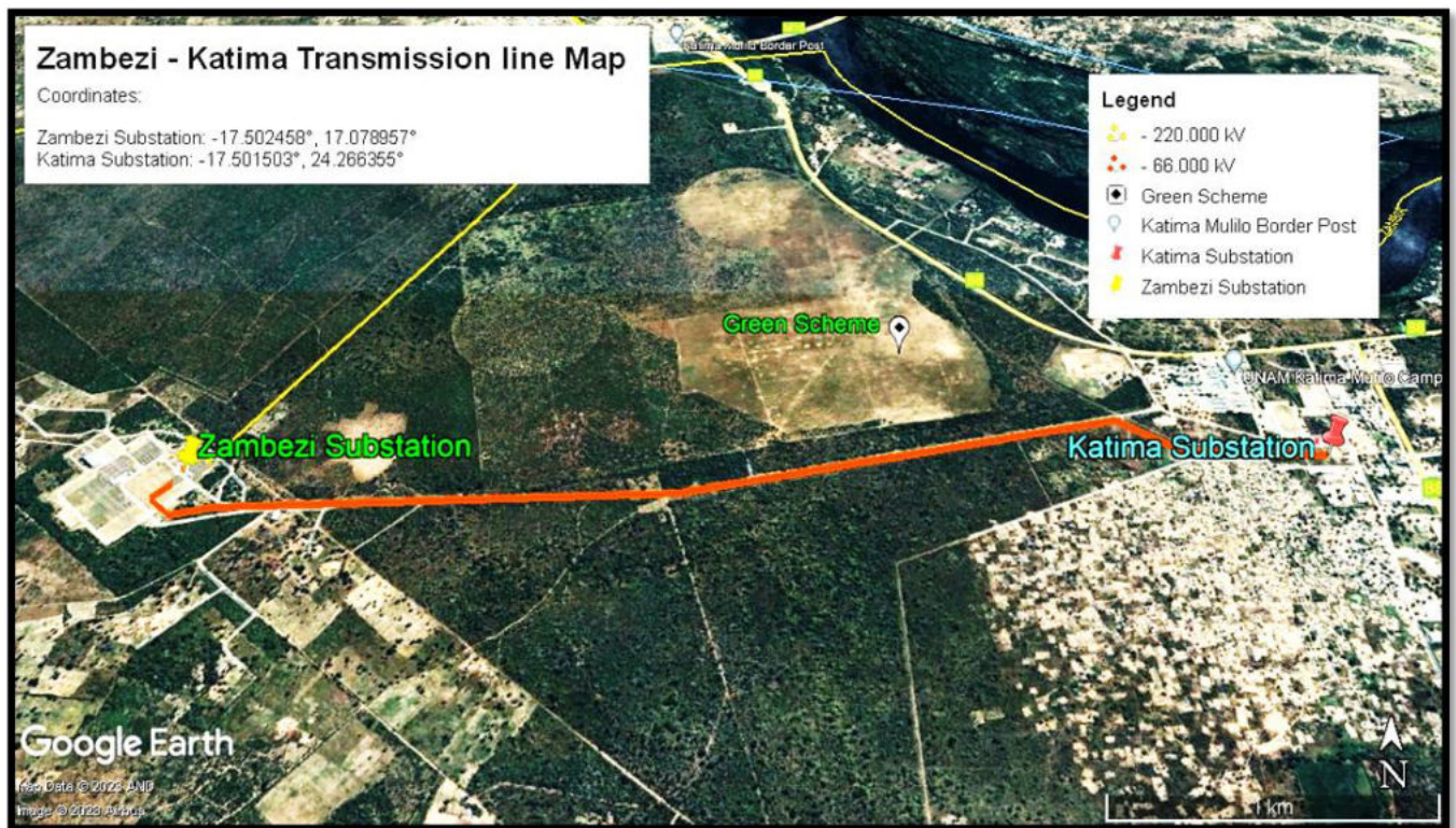
Figure 1: Locality map showing the 132 kV Zambezi – Katima transmission line
