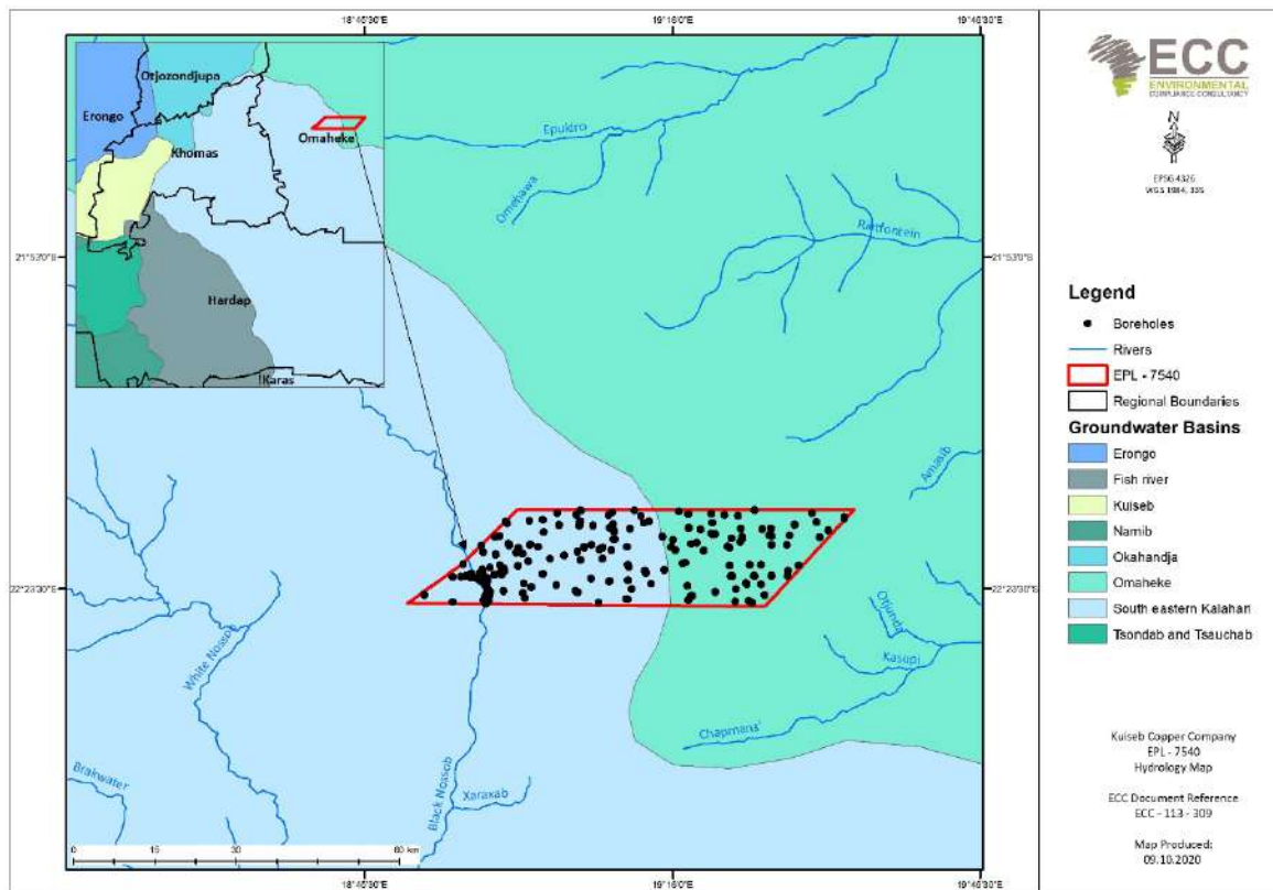
FIGURE 8 - REGIONAL HYDROLOGY MAP OF EPL 7540
