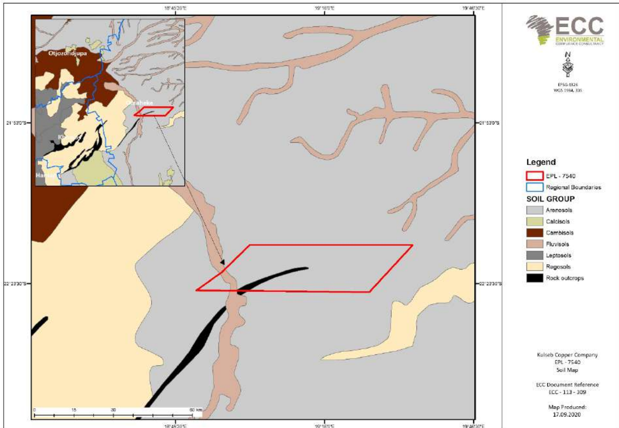
FIGURE 7 - REGIONAL SOIL MAP OF EPL 7540
