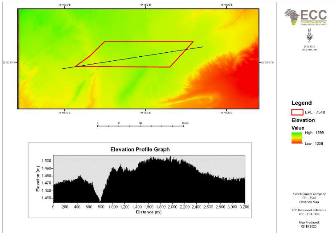
FIGURE 6 - ELEVATION PROFILE FOR EPL 7540
