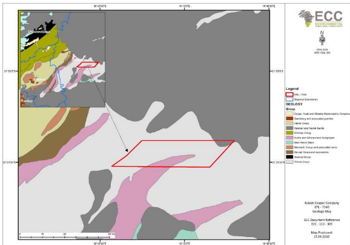
FIGURE 5 - REGIONAL GEOLOGICAL SETTING OF EPL 7540
