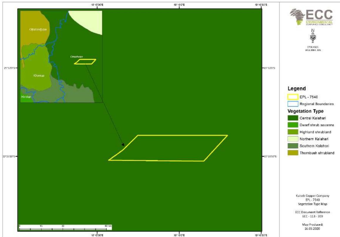
FIGURE 9 - REGIONAL VEGETATION MAP OF EPL 7540
