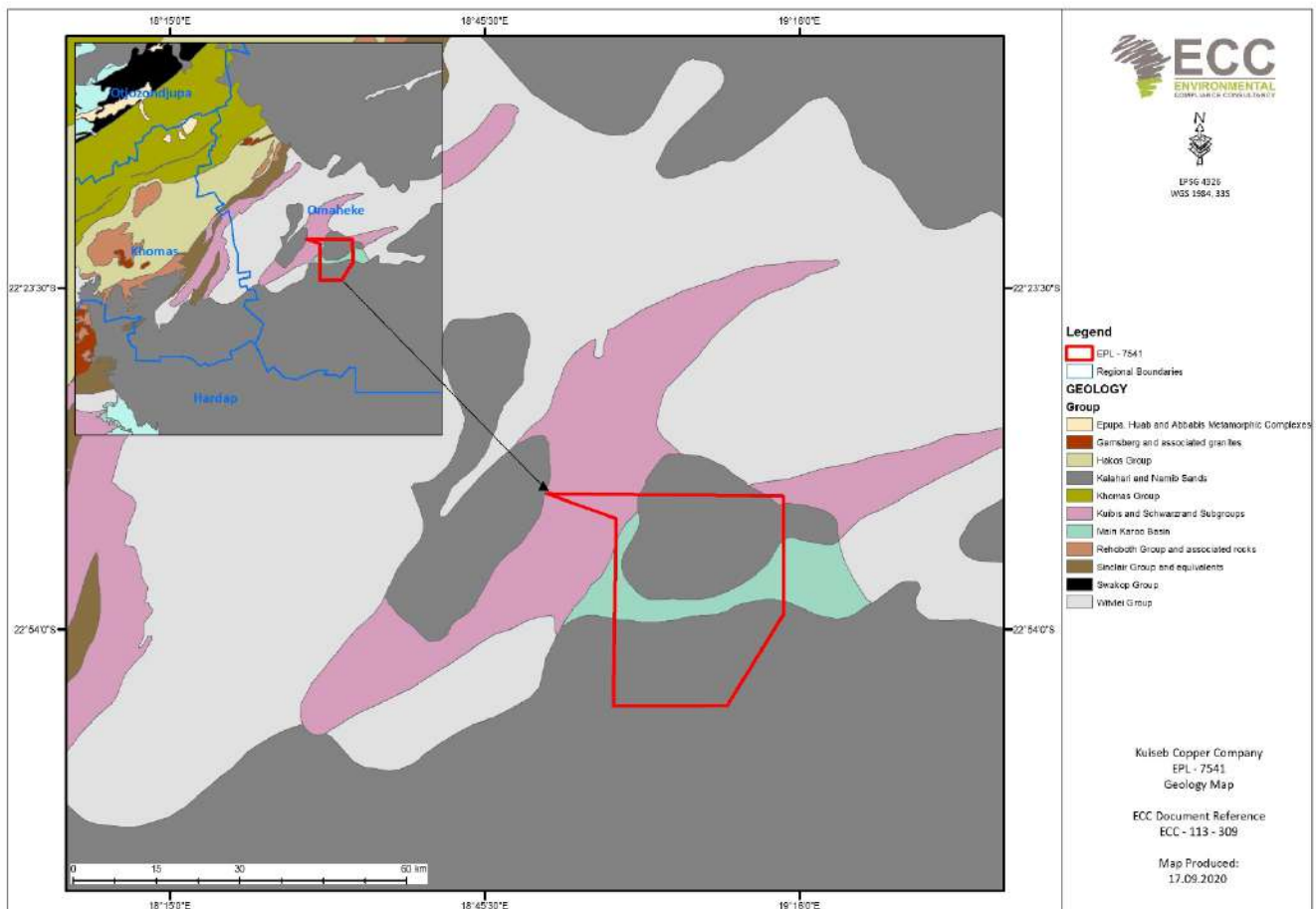
FIGURE 5 - REGIONAL GEOLOGICAL SETTING OF EPL 7541
