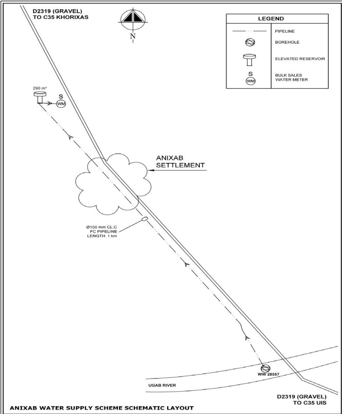
Figure 1 Anichab Scheme Layout
