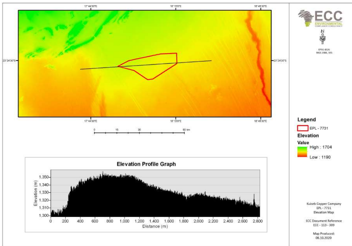
FIGURE 6 - ELEVATION PROFILE OF EPL 7731
