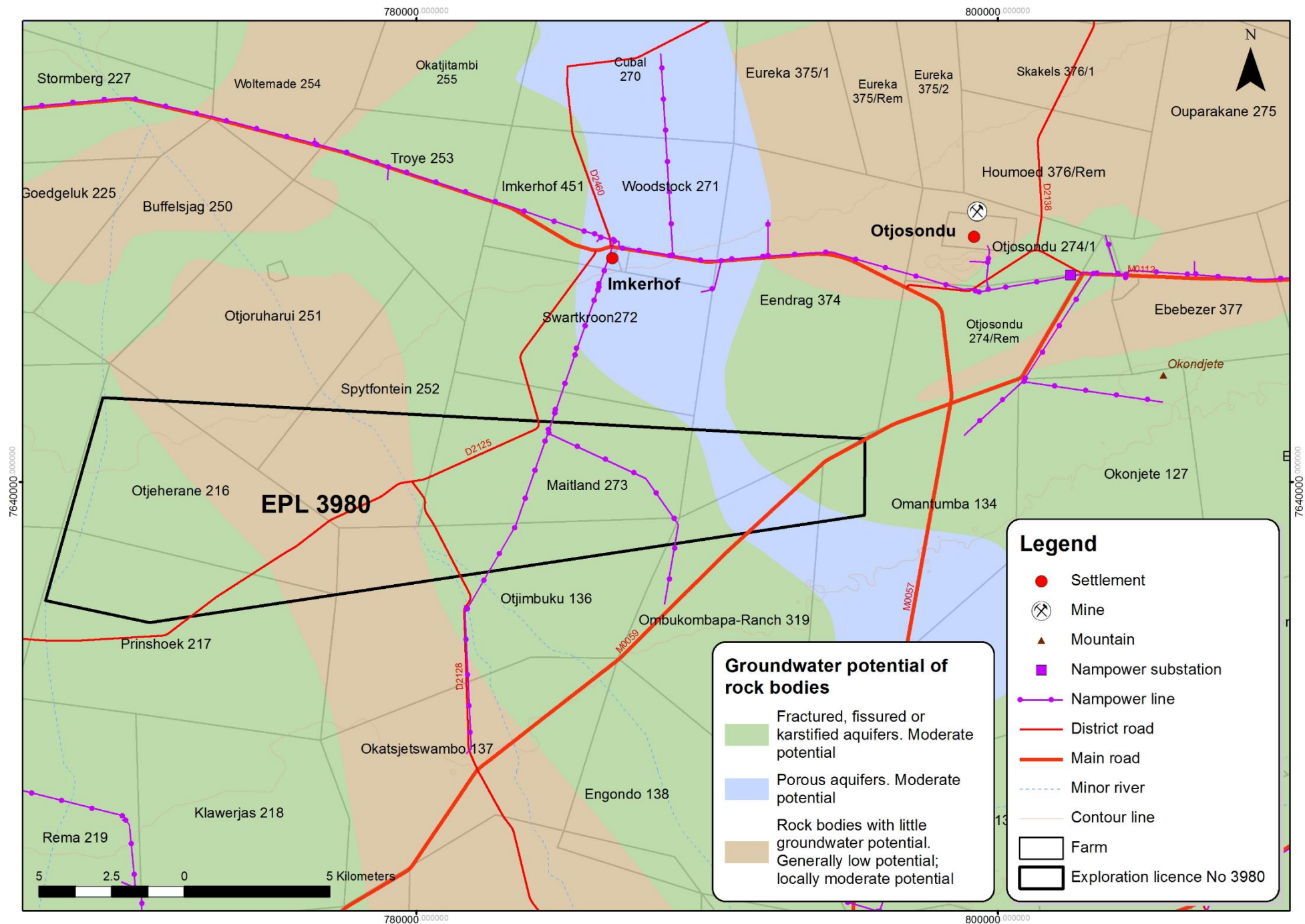
Figure 1.7: Simplified hydrogeological map of the EPL 3980 (RBS Map Prepared by Katharina Dierkes, 2020).
