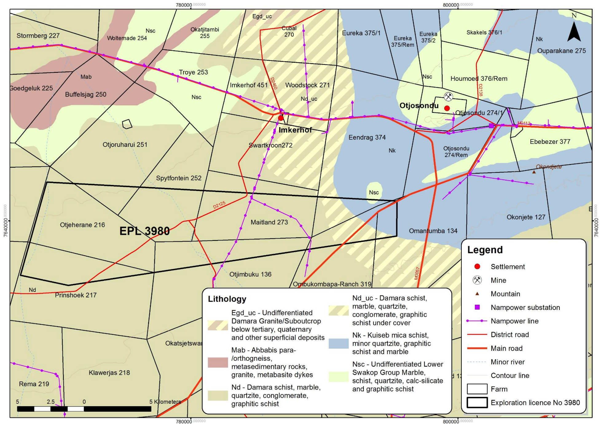
Figure 1.6: Simplified local geological map of the EPL 3980 (RBS Map Prepared by Katharina Dierkes, 2020).
