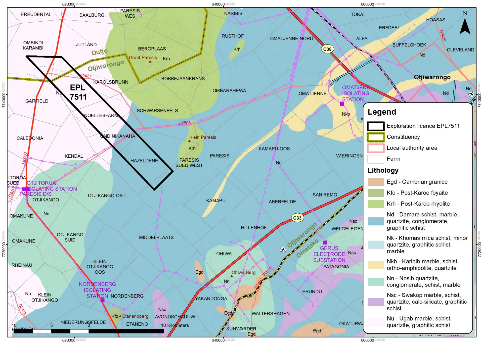
Figure 1.6: Simplified local geological map of the EPL 7511 (RBS Map Prepared by Katharina Dierkes, 2020).
