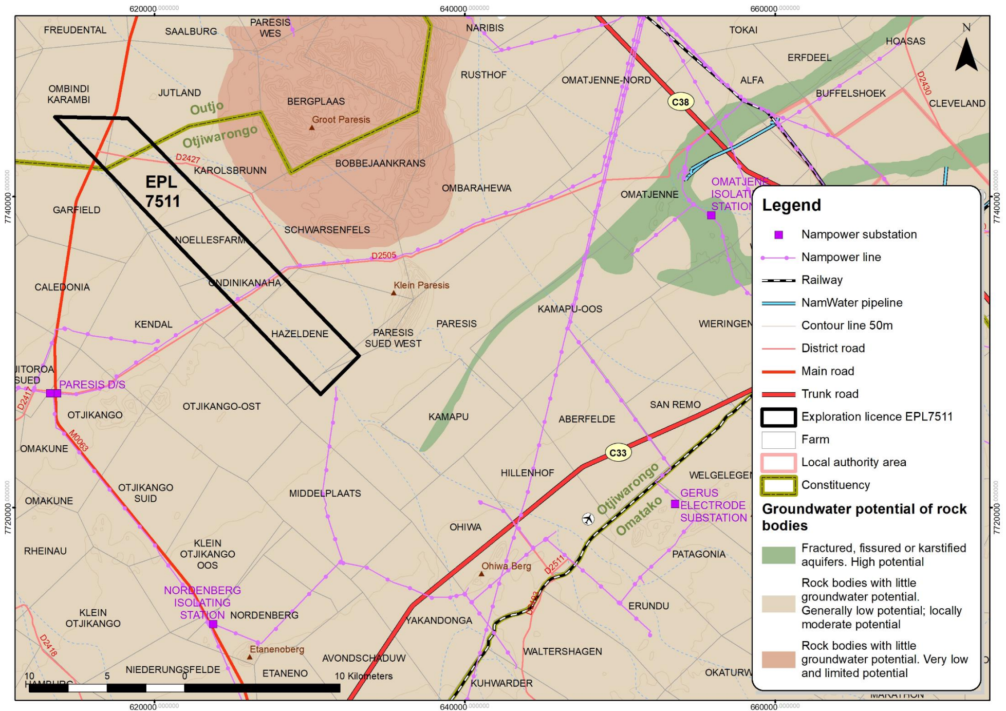
Figure 1.7: Simplified hydrogeological map of the EPL 7511 (RBS Map Prepared by Katharina Dierkes, 2020).
