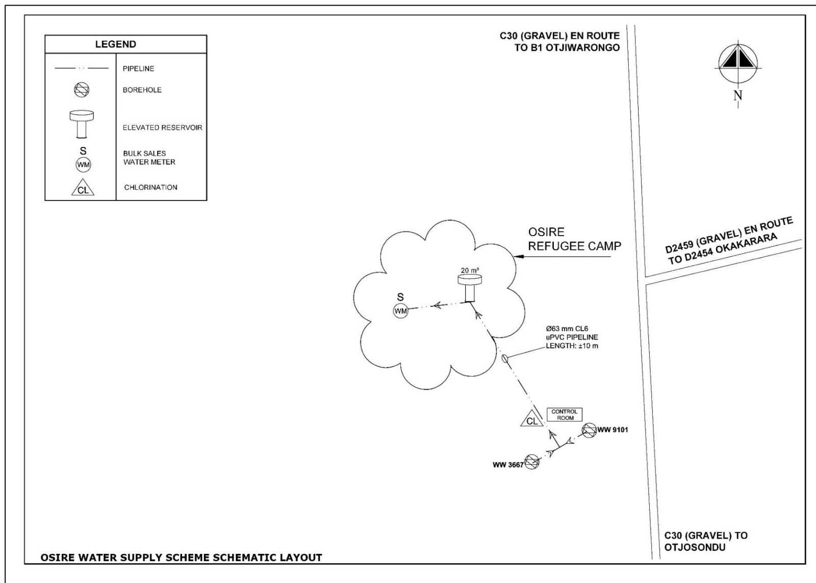
Figure 2: Osire Scheme Layout
