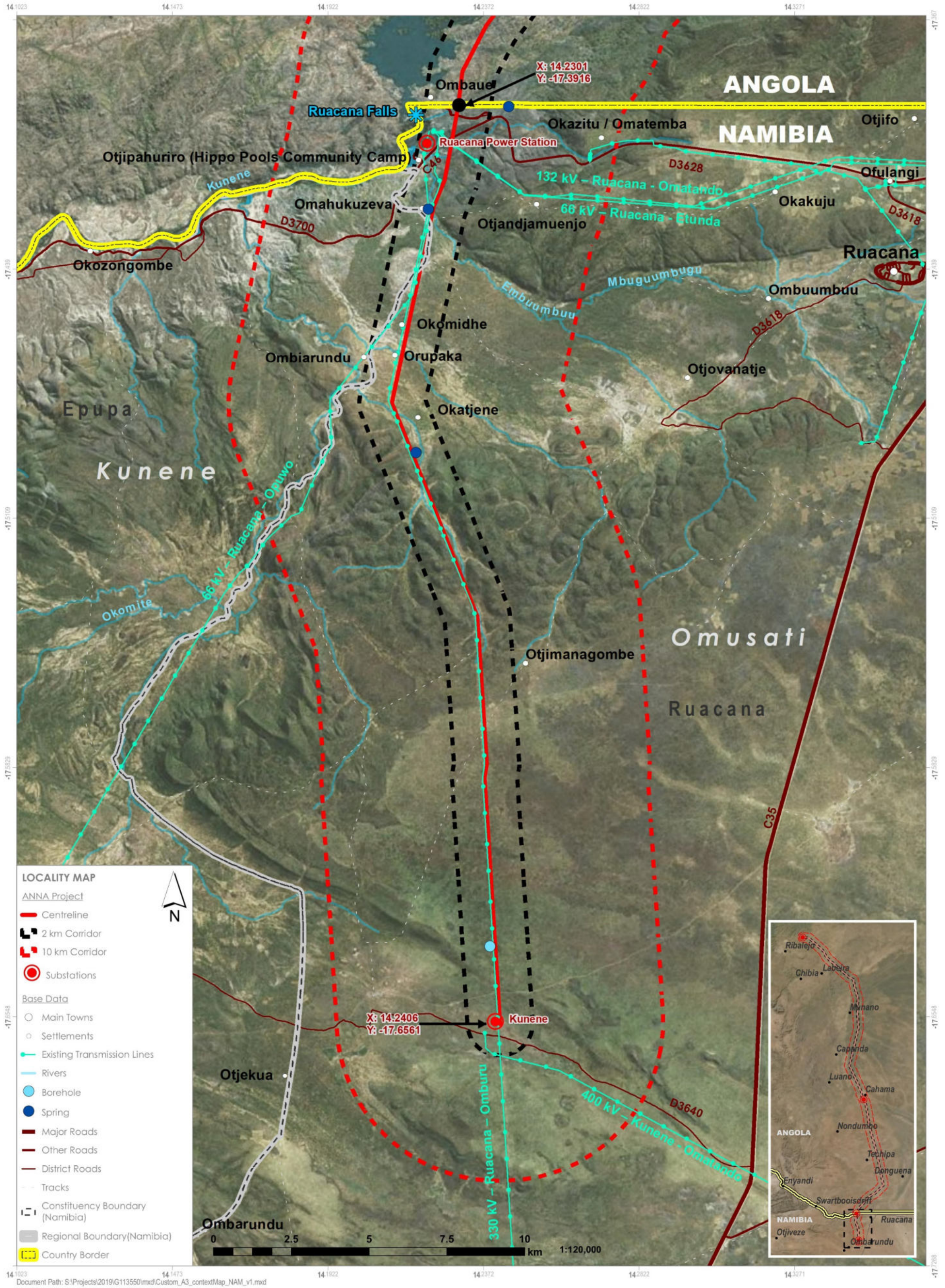
Figure 1-2: Locality map for the Namibian portion of the transmission line
