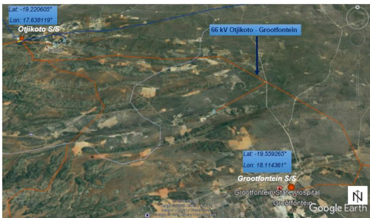
Figure 1: Map showing the 66 kV Otjikoto – Grootfontein transmission line
