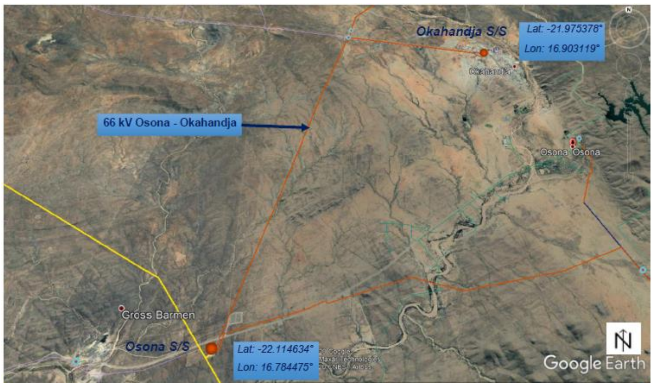
Figure 1: Map showing the 66 kV Osona – Okahandja transmission line
