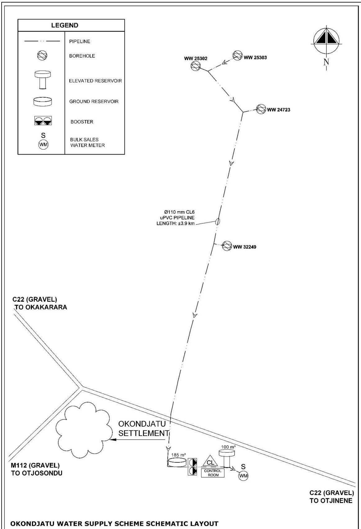
Figure 2: Okondjatu Scheme Layout
