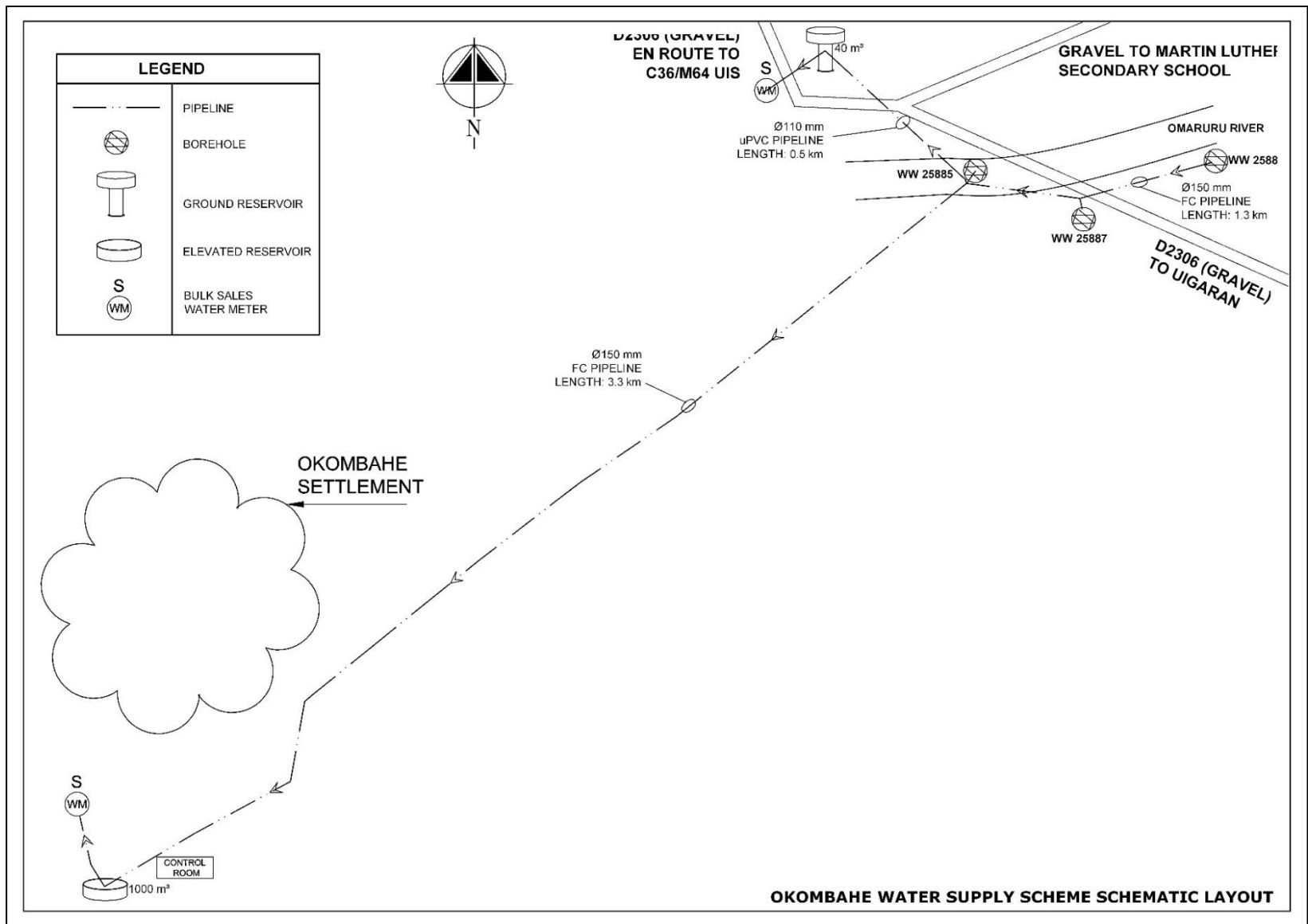
Figure 2: Okombahe Scheme Layout
