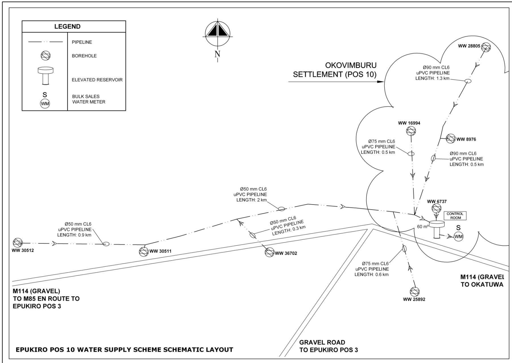
Figure 3: Epukiro Pos 10 Scheme Layout
