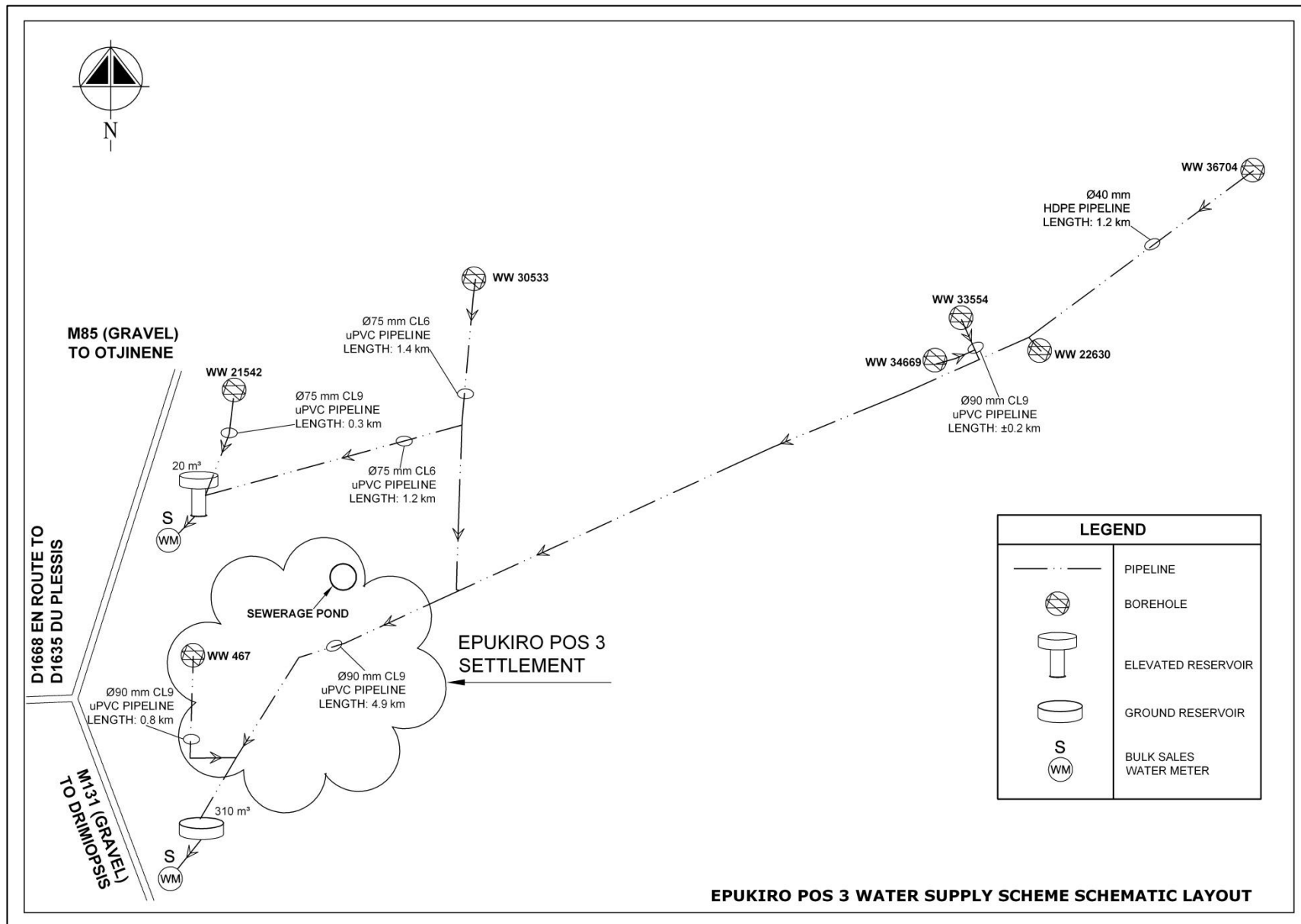
Figure 1: Epukiro Pos 3 Scheme Layout
