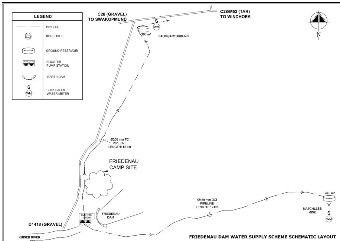
Figure 2: Friedenau Dam Scheme Schematic
