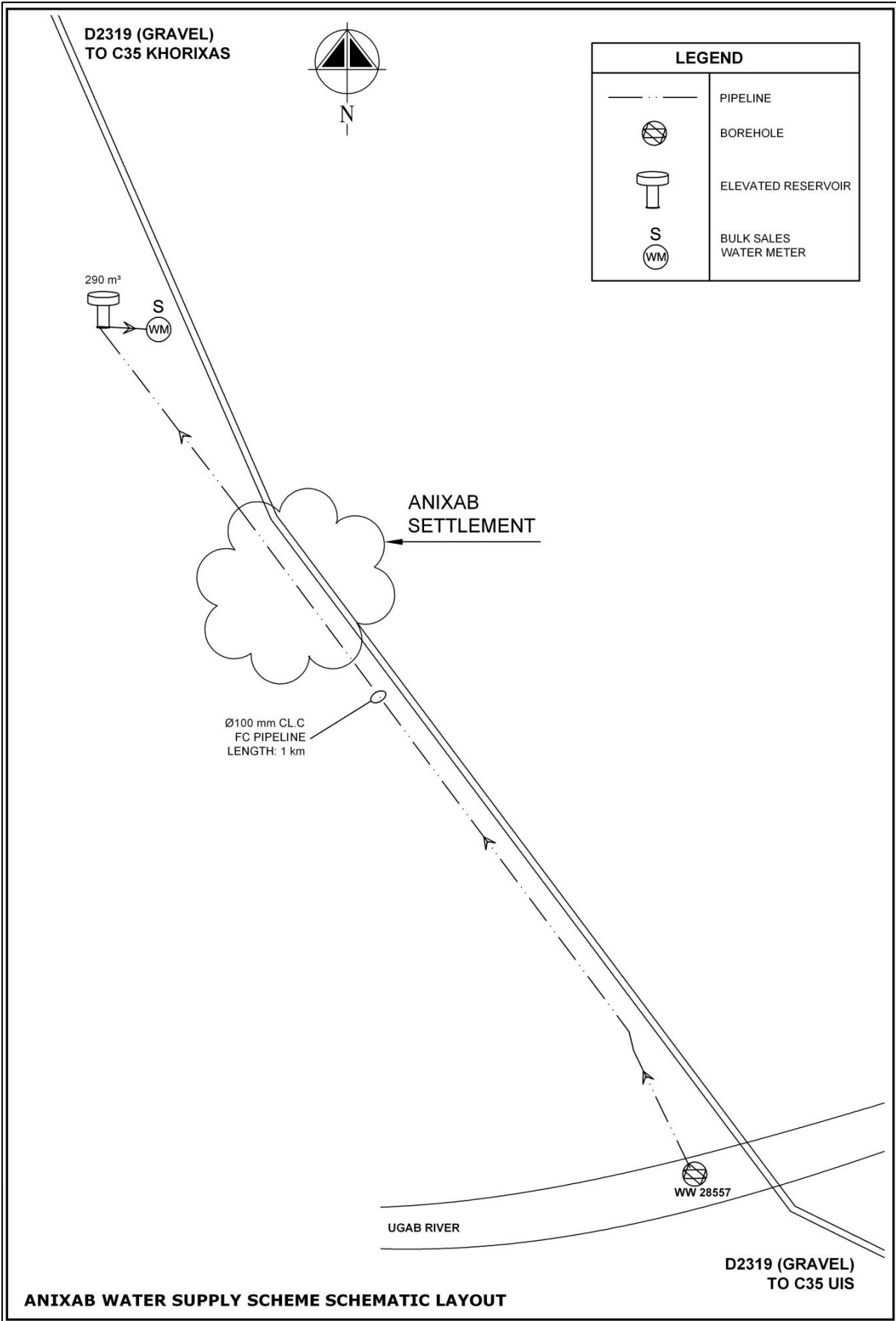
Figure 2: Anichab Scheme Layout
