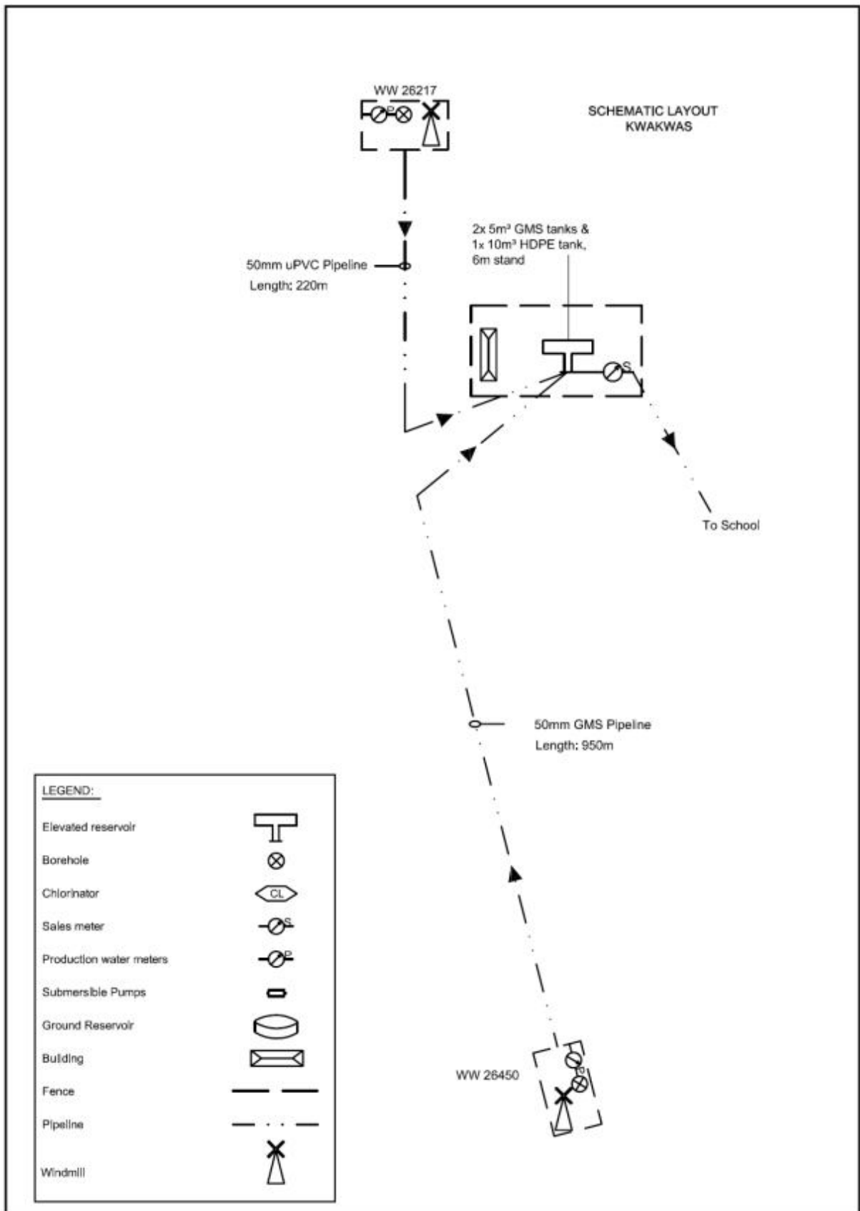
Figure 2: Kwakwas Scheme Schematic Layout
