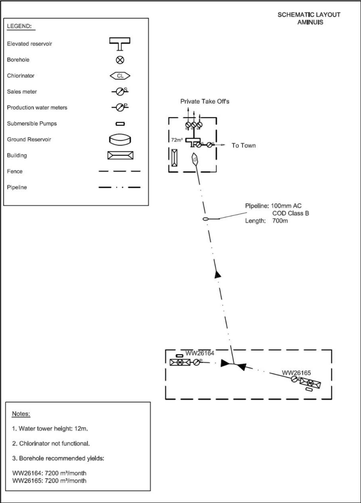
Figure 2: Aminius Scheme Schematic Layout
