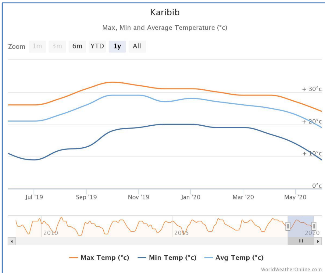
Figure 5 A graph showing the temperature patterns in Karibib, from www.worldweatheronline.com
