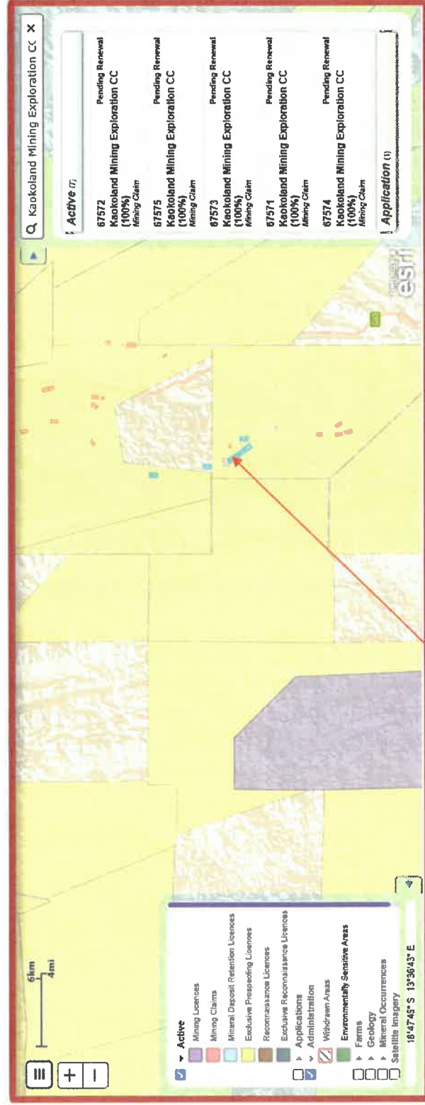
Figure 2: Location of the 7 mining claims; 67569 – 67575, situated at Otwani, Opuwo Rural Constituency, Kunene Region, Namibia (MME Portal, 2020).
