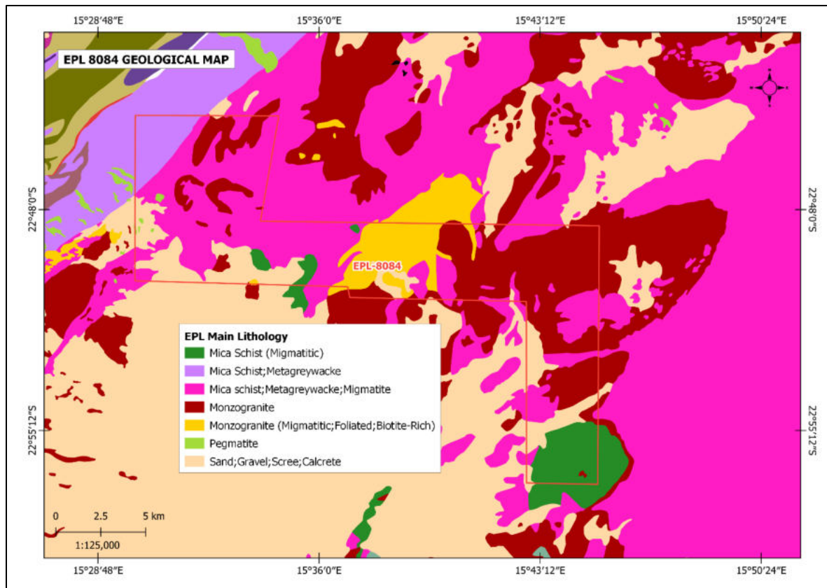
Figure 6: Geology map of EPL 8084
