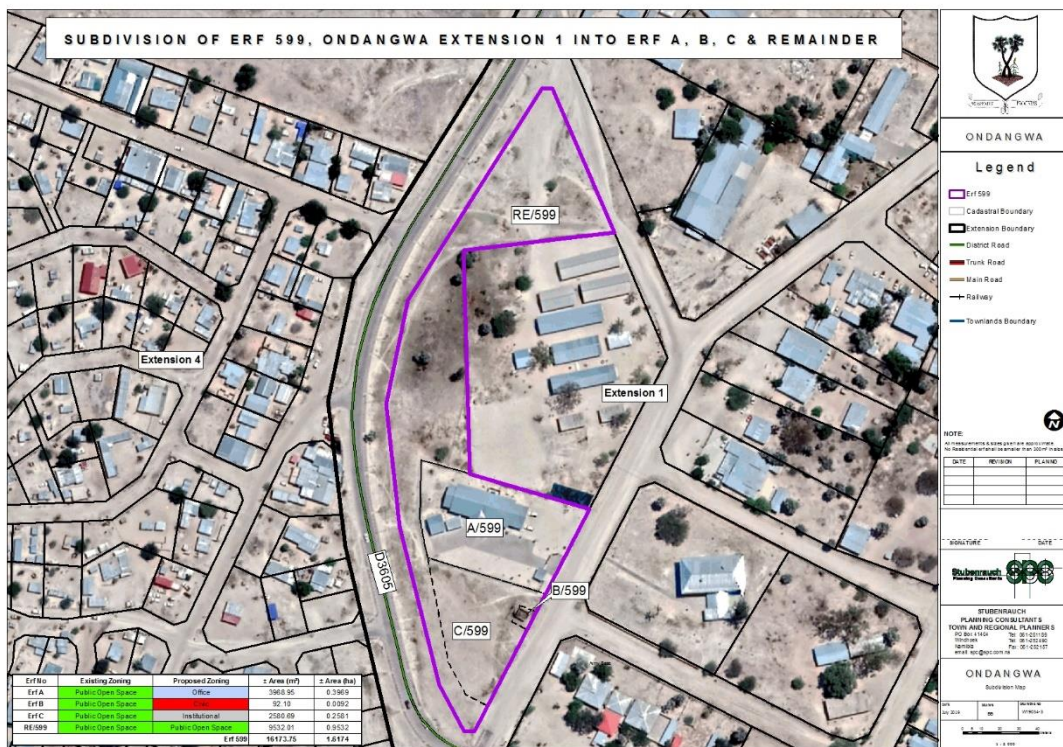
Figure 2: Subdivision of Erf 599, Ondangwa Extension 1 into Erven A, B, C and Remainder
