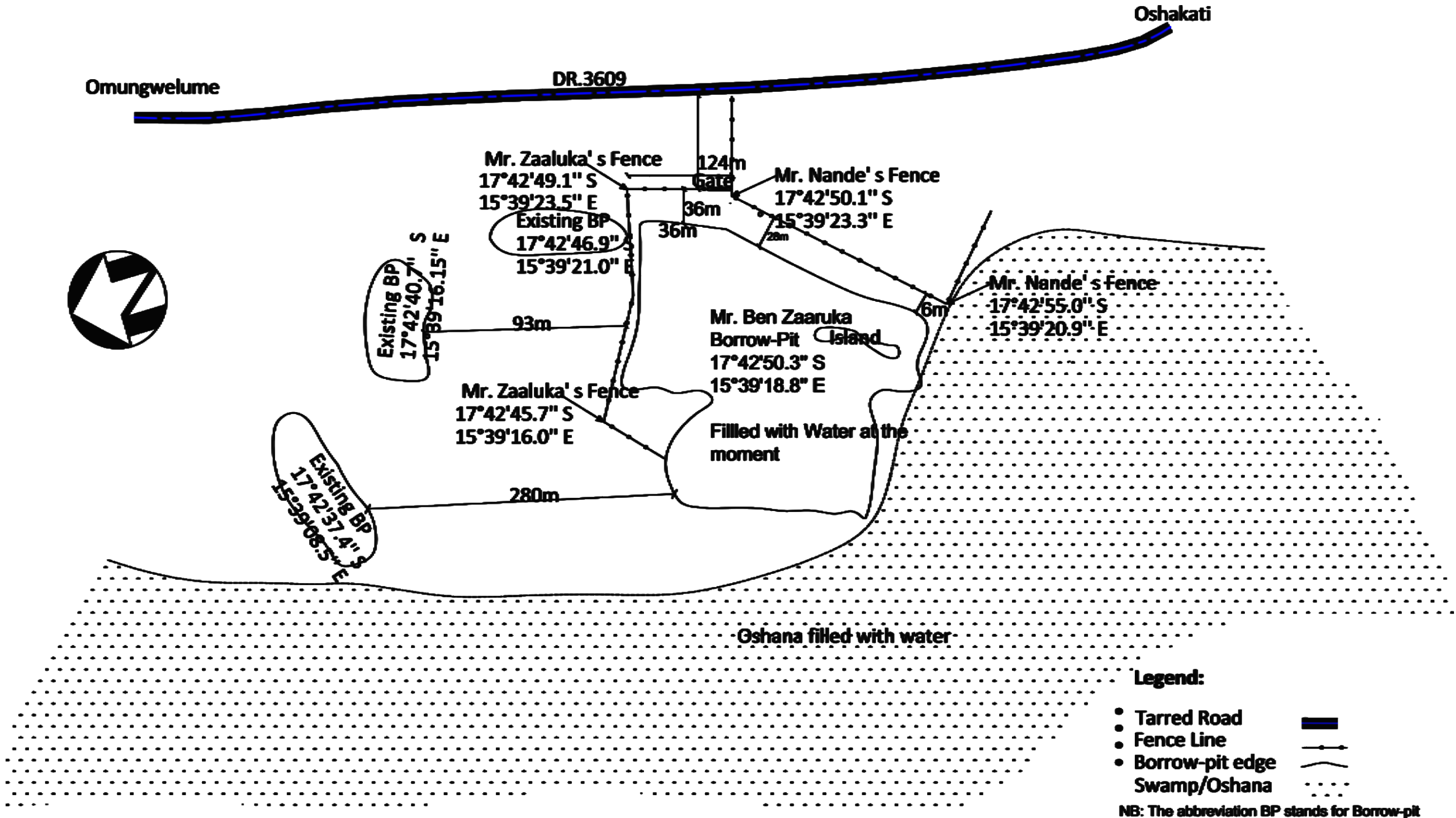
A drawing illustrating the locality of Mr. Ben Zaaruka's borrow-pit at Onanime village, 6.4 km alongside Oshakati to Omungwelume road
