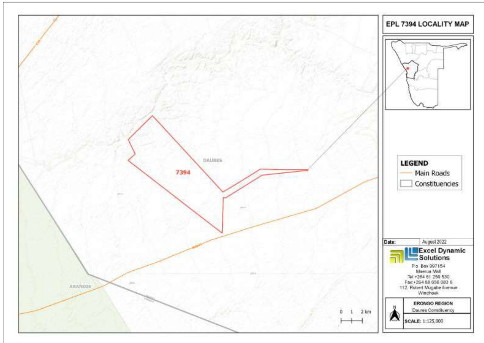
Figure 1: Location of EPL 7394 near Henties Bay in the Erongo Region
