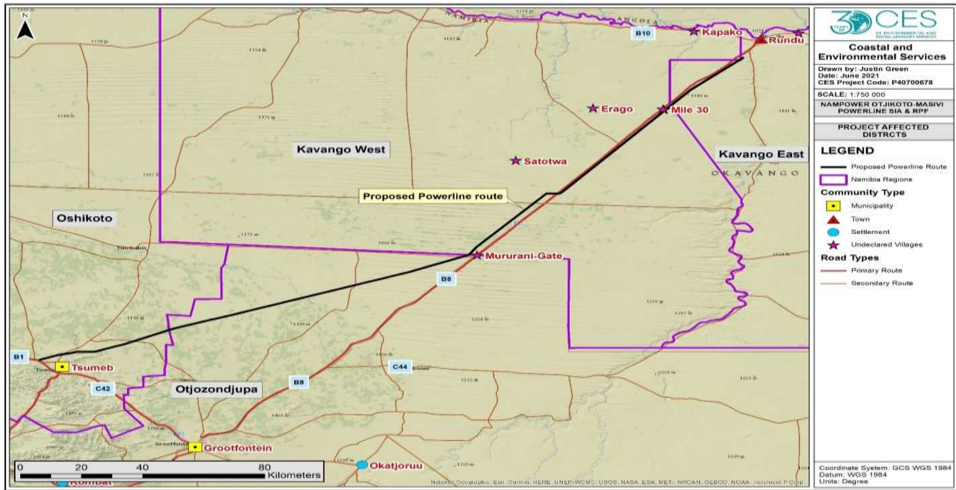
Figure 2: Proposed 220kv Transmission Line from Otjikoto Substation to Masivi Substation
