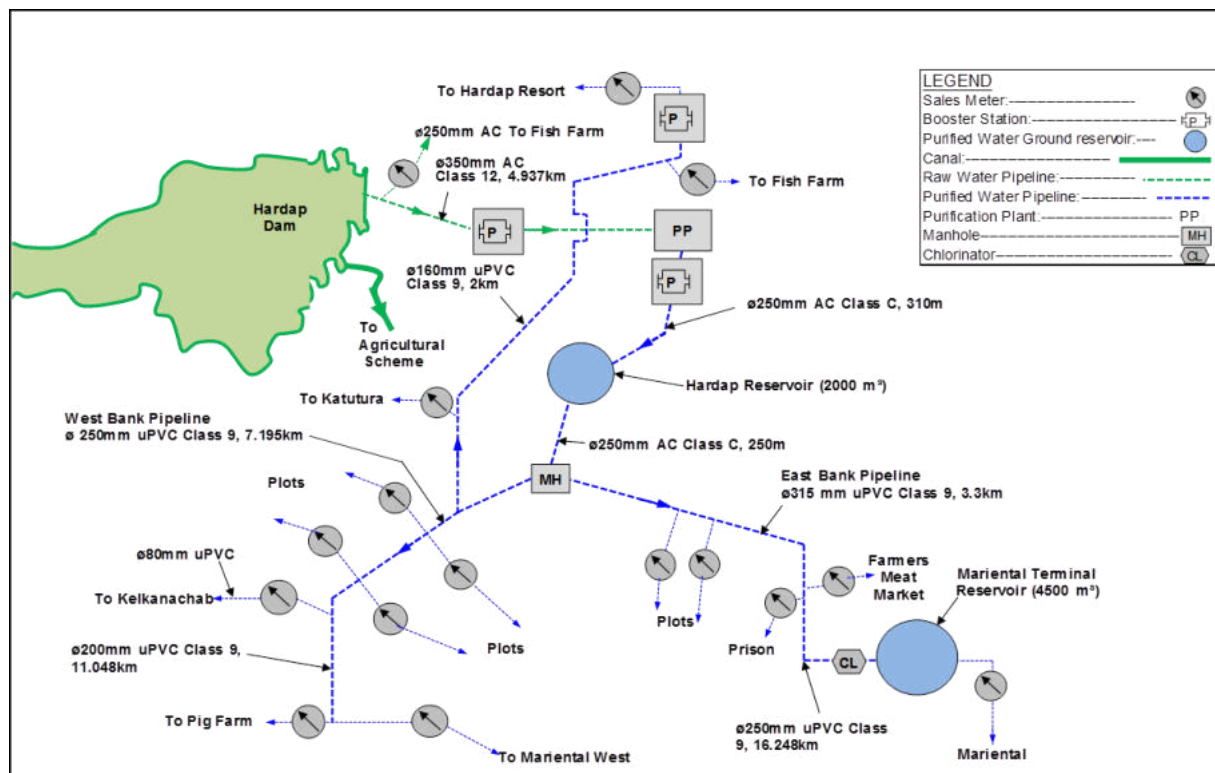
Figure 2: Hardap-Mariental Schematic Diagram
