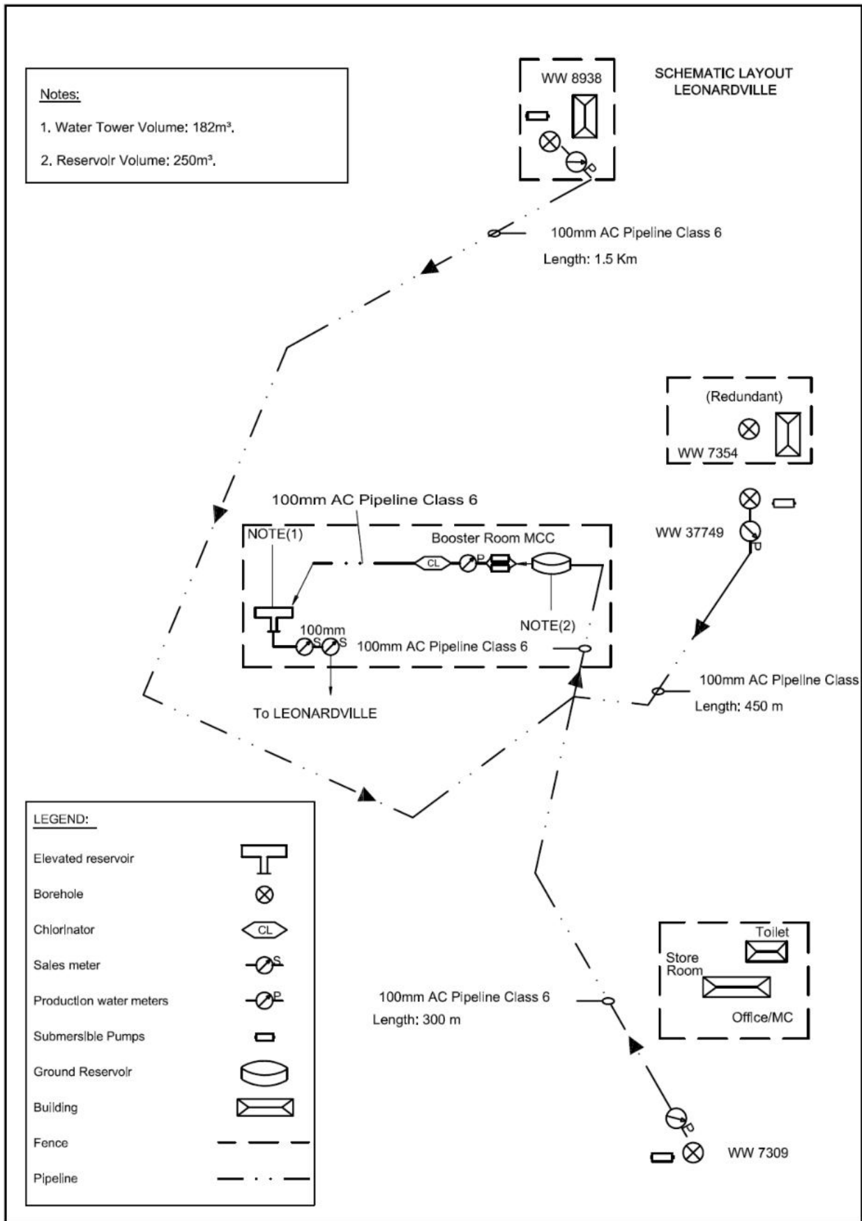
Figure 2: : Leonardville Scheme Schematic Layout
